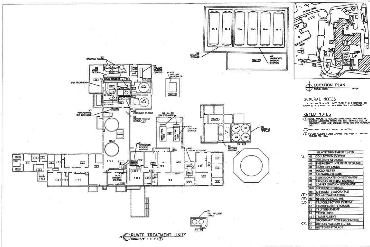
Figure 2. RLWTF Location and Treatment Units
